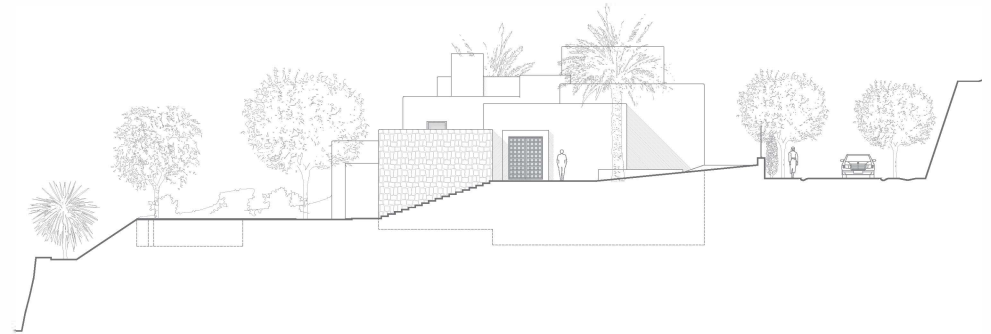
Alzado Norte / North Elevation
